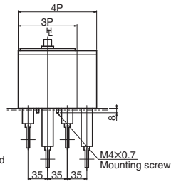
Drilling plan (front view)
